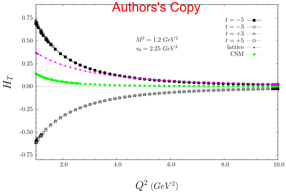
Figure 3: The dependence of H_T on Q^2 at M^2 = 1.2 GeV^2 and s_0 = 2.25 GeV^2 and four fixed values of t : t = -5; -3; 3; 5 , for the isoscalar current.
