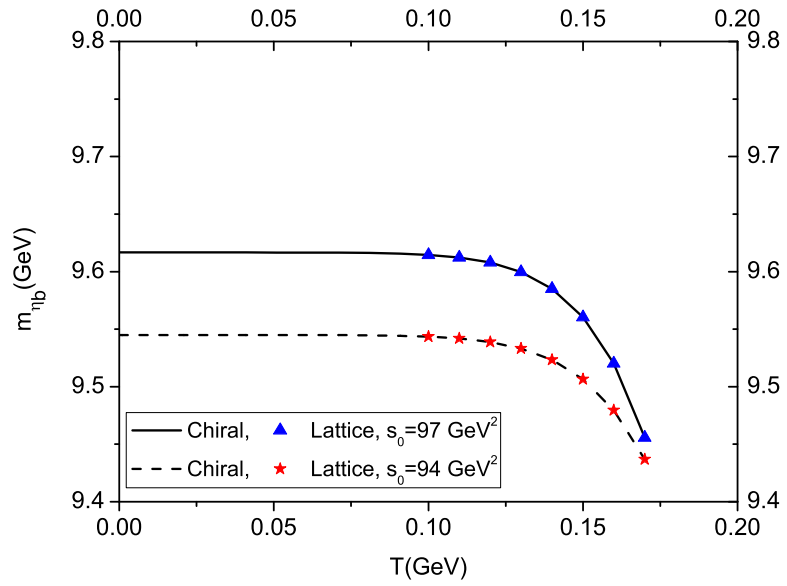
FIG. 5. The same as Fig. 1 but for m_{\pi_b} .
